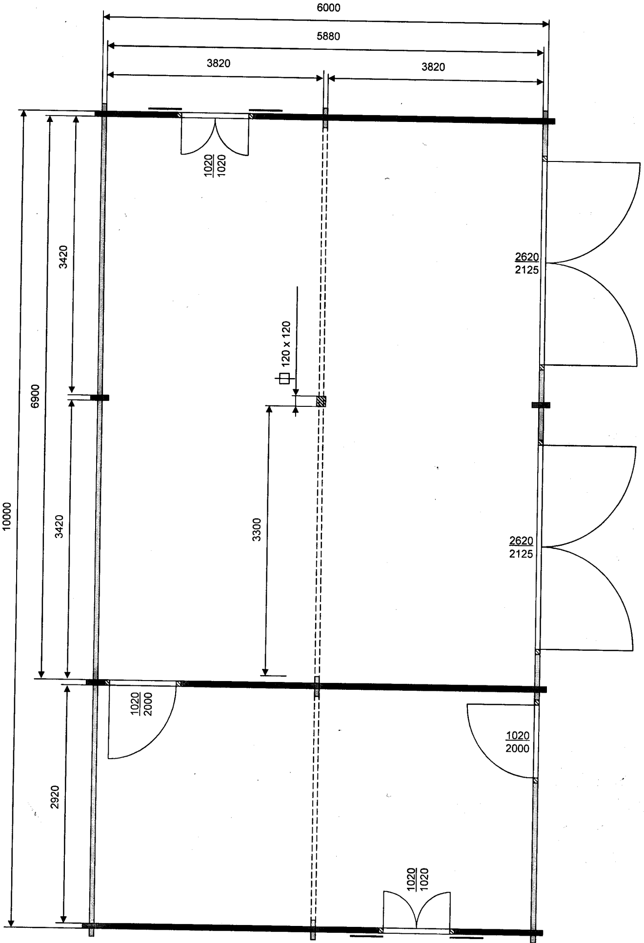
PLAN GARAJ TIP "GAR-2-MEGA"
